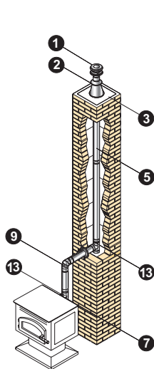
Masonry Chimney Relining
