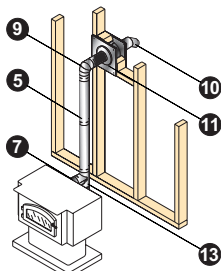
Through-The-Wall Vertical Rise
