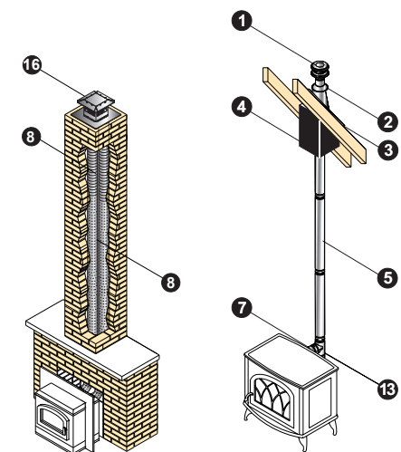
Co-Linear SS Flex Installation for Pellet Inserts
