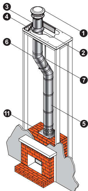
Masonry Firebox with Metal Chimney
