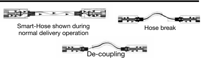
Smart-Hose shown in failure situations, instantly shutting down the flow
