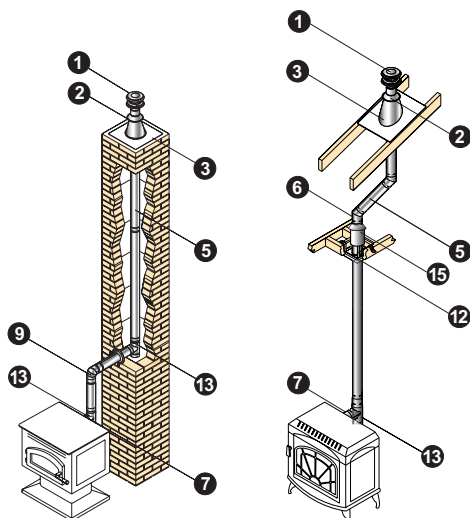
Masonry Chimney Relining
