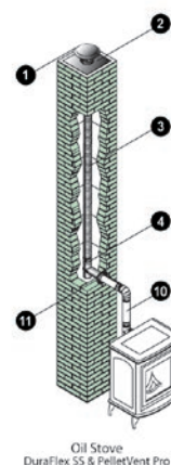
Oil Stove DuraFlex SS & PelletVent Pro
