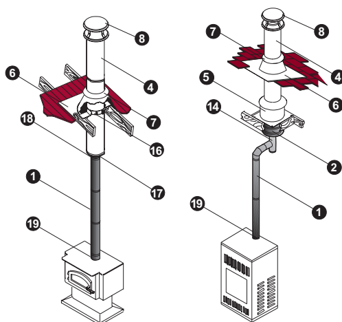
Cathedral Ceiling
